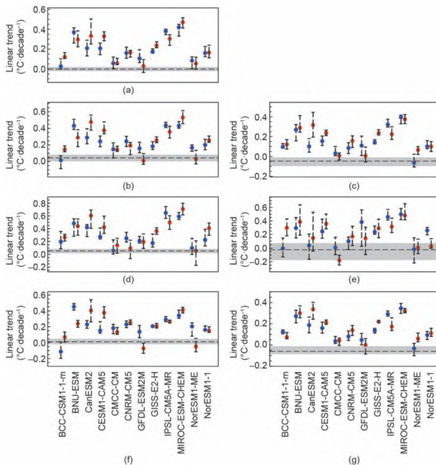
Fig. 3. Weighted linear trend ( ^{\circ}\text{C}\cdot\text{decade}^{-1} ) in the models for the (a) globe, (b) NH, (c) SH, (d) NH land, (e) SH land, (f) NH ocean, and (g) SH ocean from 2001 to 2013 under RCP4.5 (blue circles) and RCP8.5 (red circles). The dashed line indicates the value of the trend from HadCRUT4 reanalysis, and the shaded area covers the 50% confidence interval. Error bars show the 50% confidence interval for each model.
